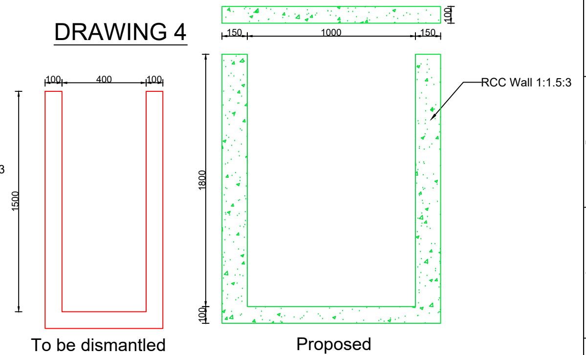
DRAWING 4 To be dismantled Proposed Dismantling of existing drain and reconstruction of new drain Location: From Mini Substation to PWD drain near boundary (35 mtr)
