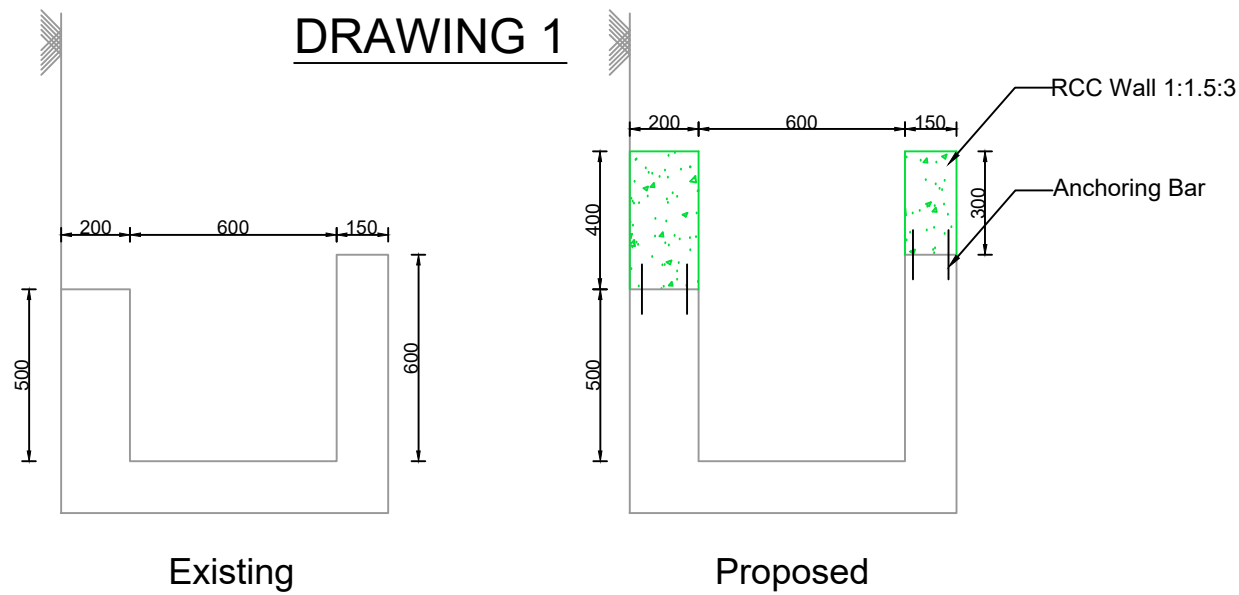
DRAWING 1 Existing Proposed Height raising of existing RCC drain Location: From KSIDC pond side to 1st boundary wall corner (14.50mtr)
