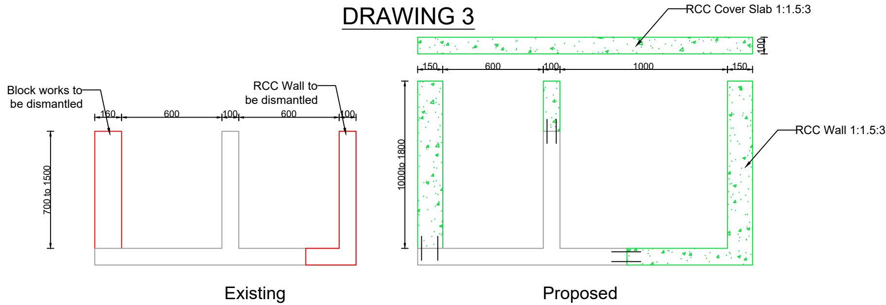
DRAWING 3 Existing Proposed Height raising and widening of existing RCC drain cum duct Location: From cross culvert near STP to cross culvert in front of Mini substation (89 mtr)
