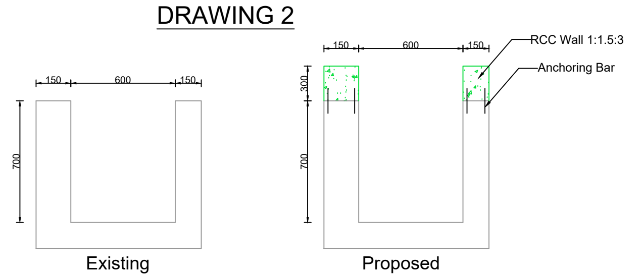
DRAWING 2 Existing Proposed Height raising of existing RCC drain Location: From 1st boundary wall corner to cross culvert near STP (76.50mtr)
